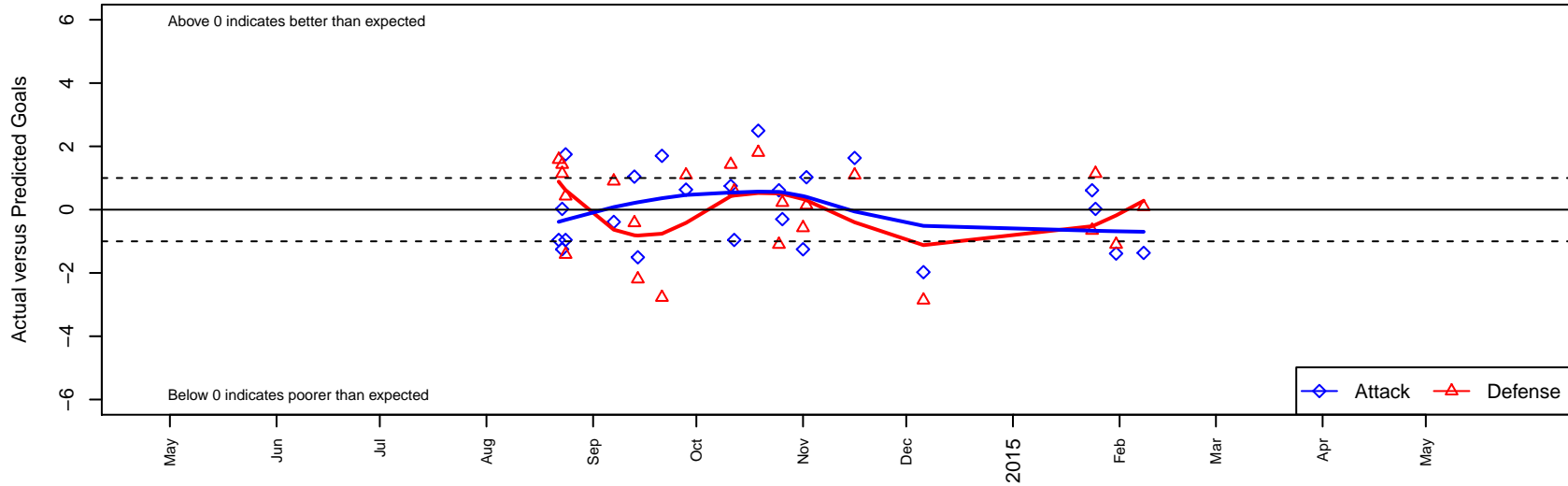
3 Rivers Black B97 Dots are actual minus expected GF (blue circles) and GA (red triangles). Blue line is smoothed change in attack strength. Red is smoothed change in defense strength.
